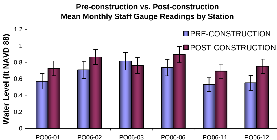
Figure 12. Mean of monthly staff gauge readings at the six staff gauges located in the Fritchie Marsh (PO-06) project area during the pre-construction (3/98-2/01) and post-construction (3/01-6/05) periods.
