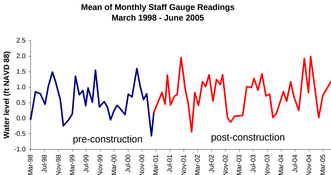
Figure 13. Mean of monthly readings from six staff gauges located in the Fritchie Marsh Restoration (PO-06) Project area from March 1998 to June 2005.
