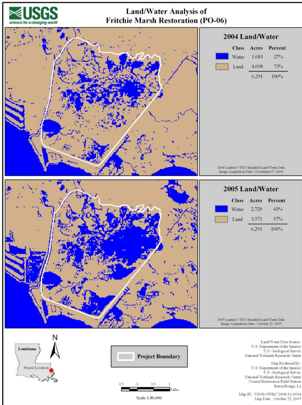
Figure 5. 2004 and 2005 land/water comparison of the Fritchie Marsh Restoration (PO-06) project area using Landsat 5 satellite imagery. The 2005 imagery was acquired two months after the passage of Hurricane Katrina.
